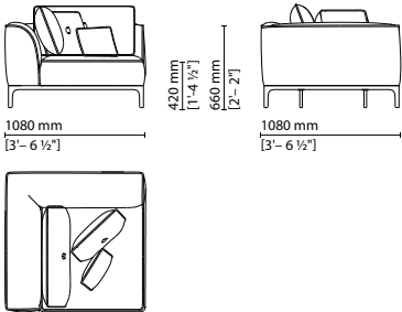
006 035 — Left corner element
