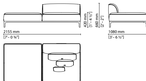
006 015 — Central element with ottoman on the left side
