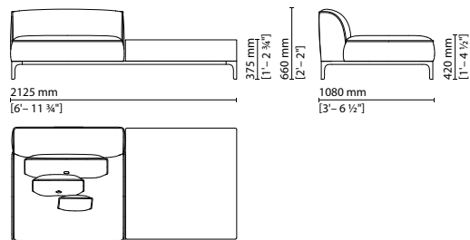
006 019 — Central element with large side table on the right
