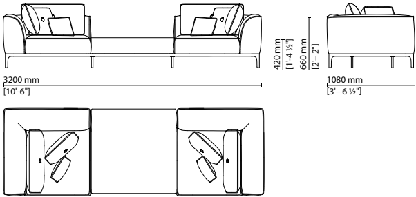
006 033 — 3 seats with central table
