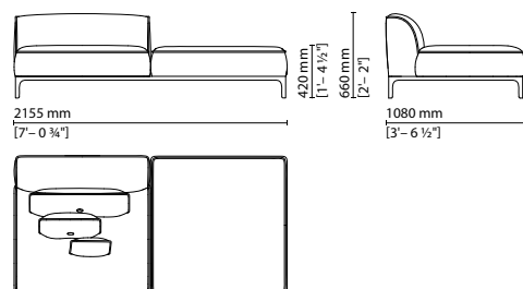
006 014 — Central element with ottoman on the right side
