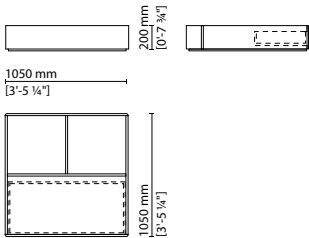
006 800 — Table with Drawer and Compartments
