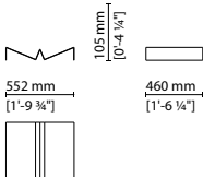
006 901 — Bar cup holder
