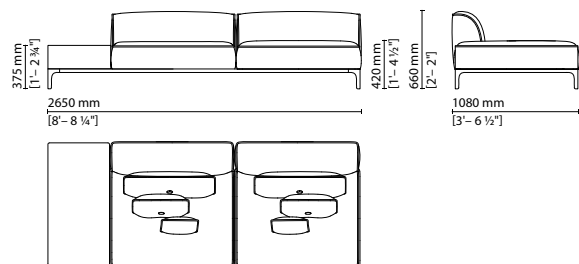
006 024 — 2-seater sofa with small side table on the left
